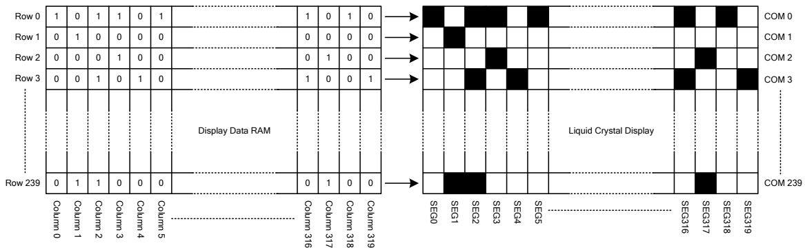
Figure 15 DDRAM Mapping
