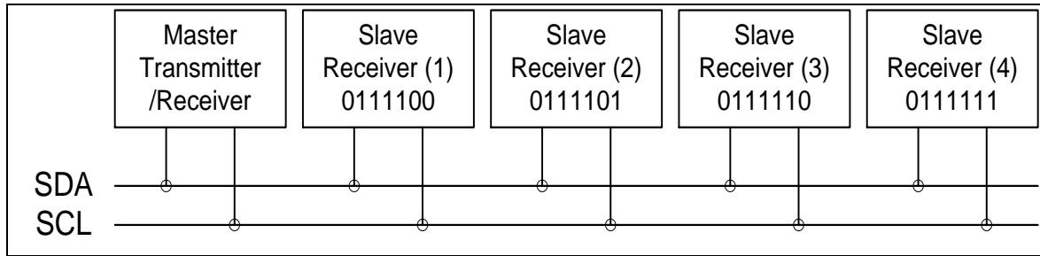
Figure 12 System Configuration
