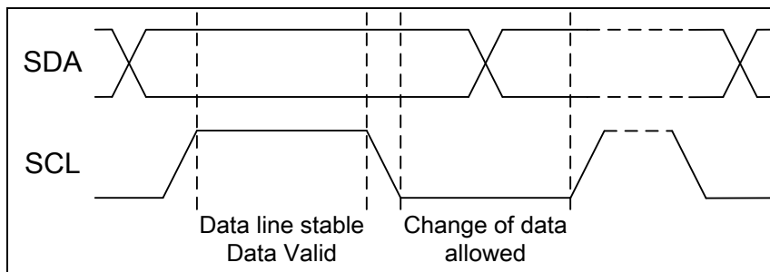
Figure 10 Bit Transfer
