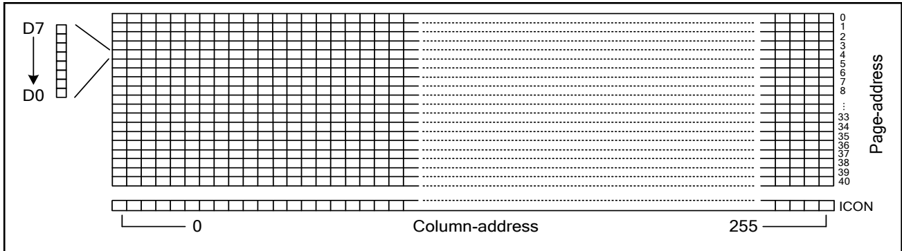
Figure 20 RAM format and addressing, if DO=0 (4-Level Gray Scale Mode)
