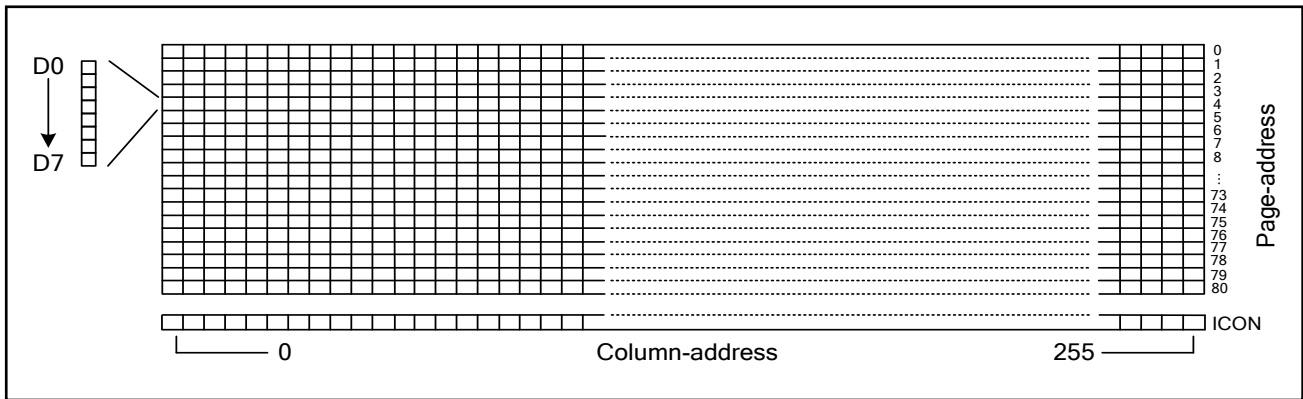
Figure 23 RAM format and addressing, if DO=1 (16-Level Gray Scale Mode)
