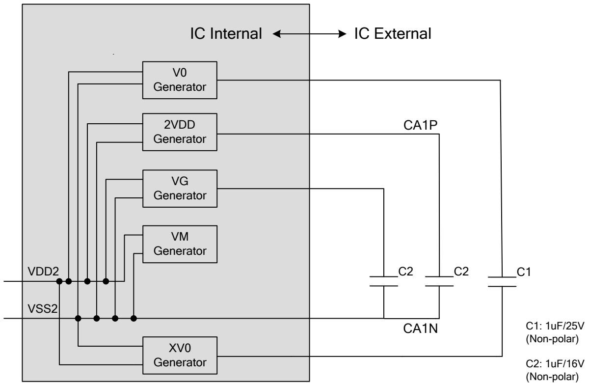
Figure 27 Power Circuit
