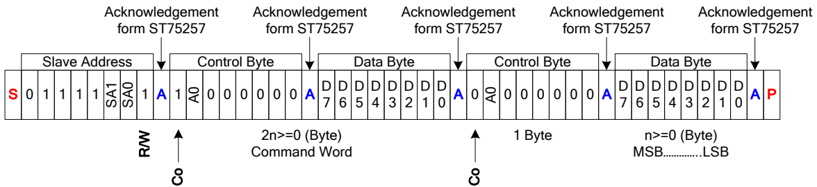
Figure 15 I 2 C Interface Protocol
