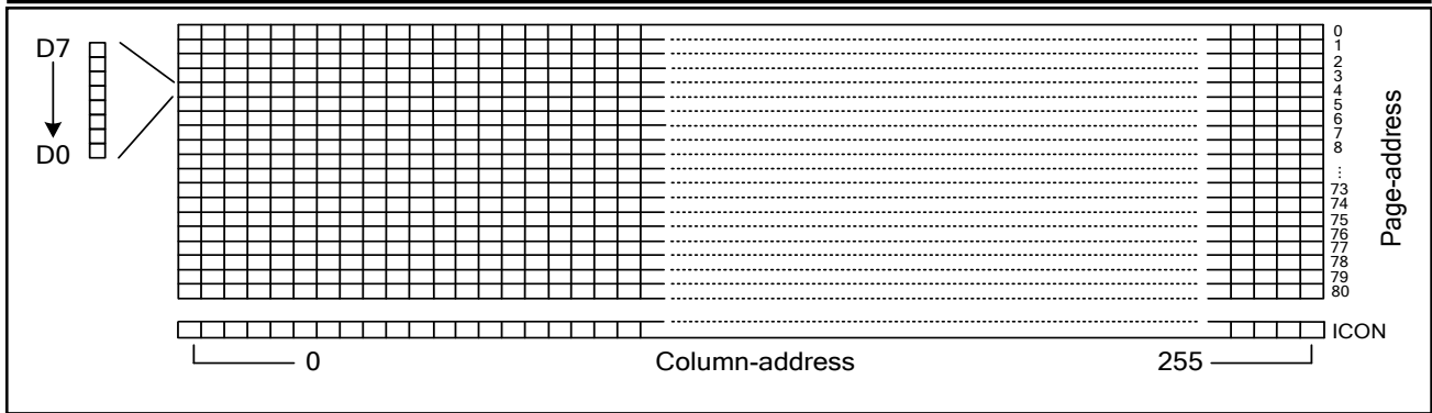
Figure 22 RAM format and addressing, if DO=0 (16-Level Gray Scale Mode)
