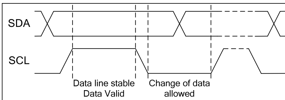
Figure 11 Bit Transfer
