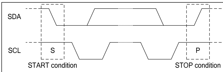
Figure 12 Definition of START and STOP Condition
