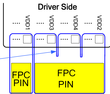
Dual VDD: VDDI and VDDA separately
