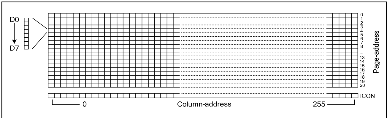
Figure 23 RAM format and addressing, if DO=1 (Monochrome Mode)
