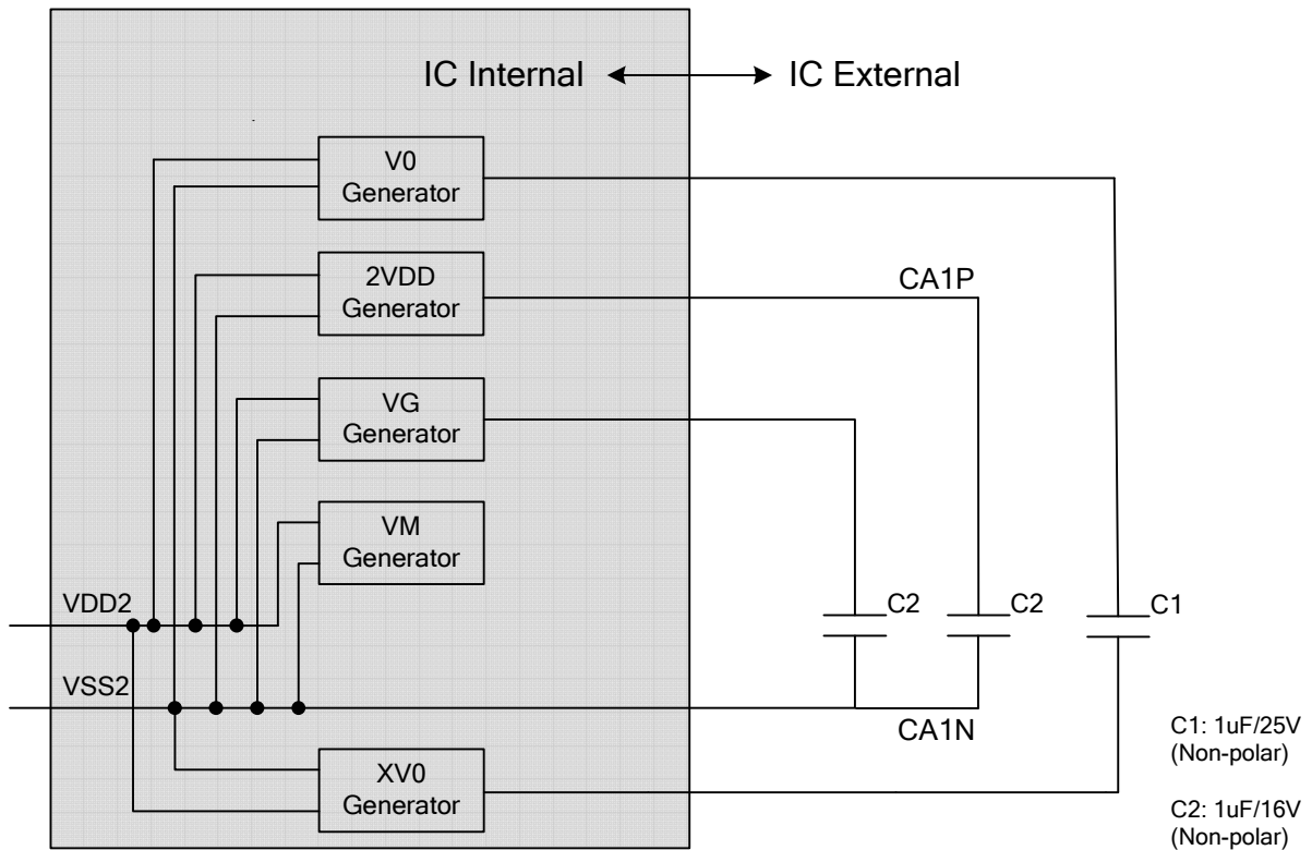
Figure 27 Power Circuit
