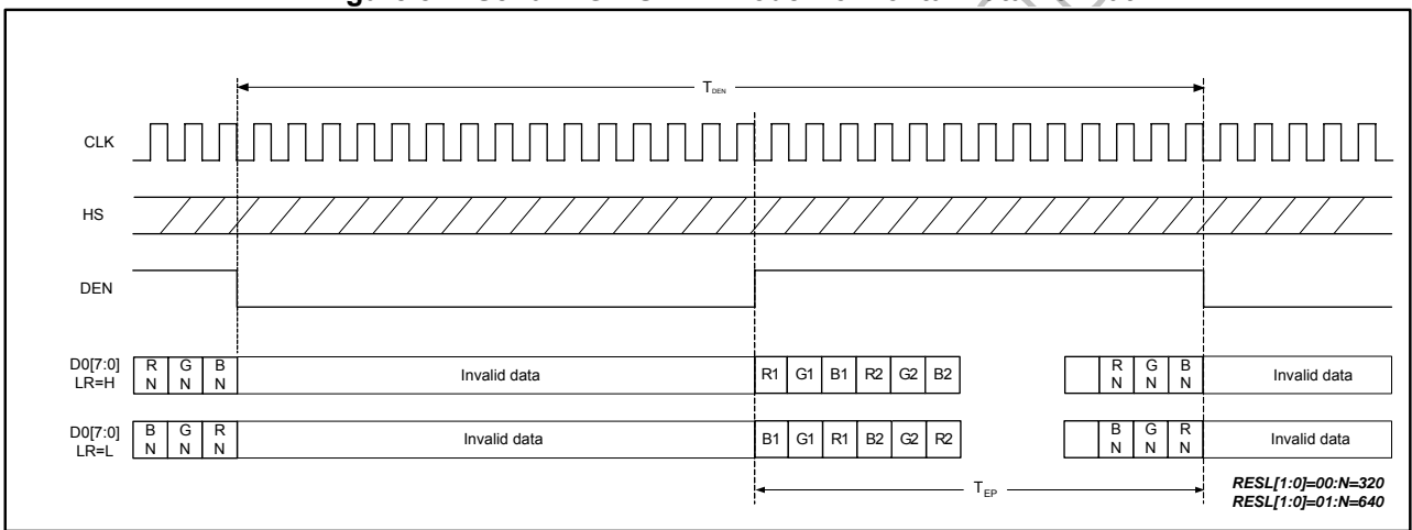
Figure 8. 3 Serial RGB DE Mode Horizontal Data Format
