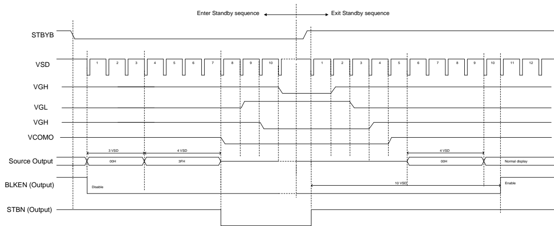
Enter and Exit Standby Mode Sequence
