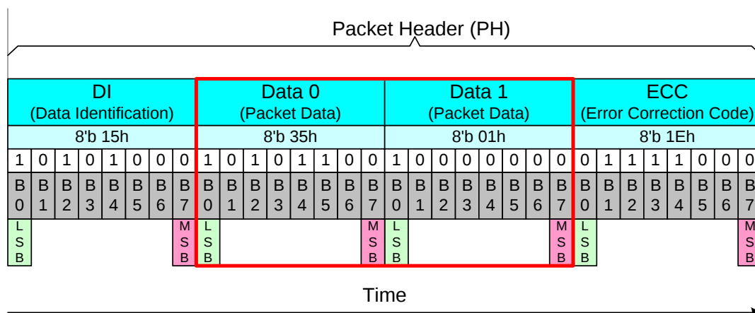
Figure 52: Packet Data (PD) of a Short Packet, 2 Bytes Information
