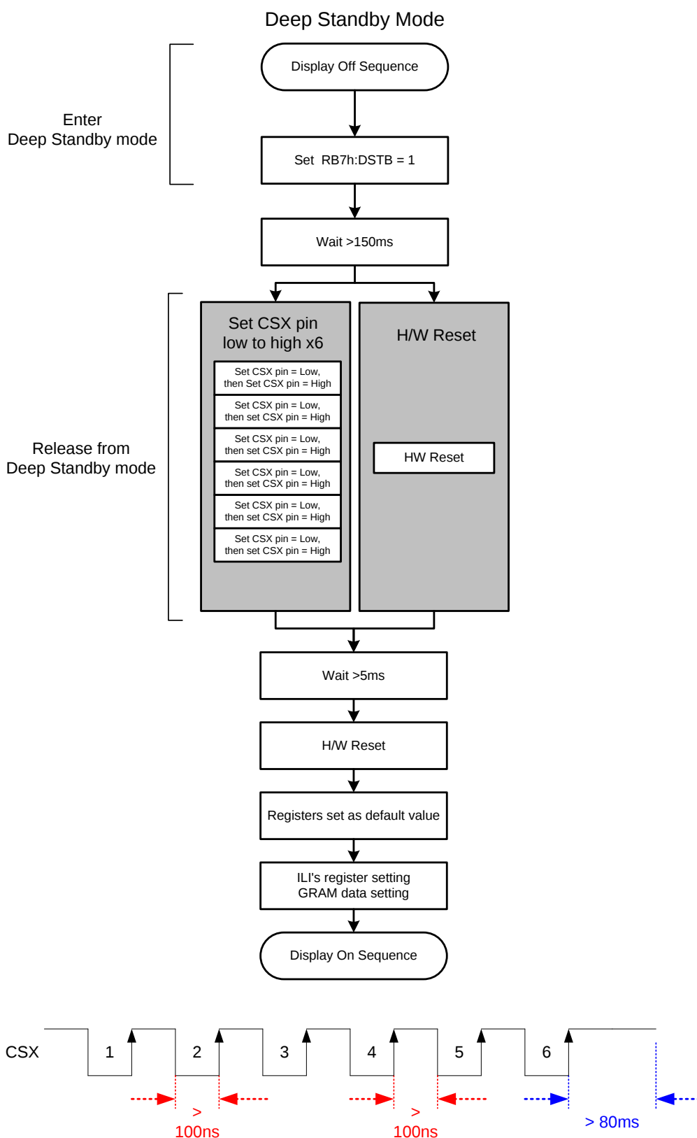
Figure 141: Deep Standby Mode Entry/Exit
