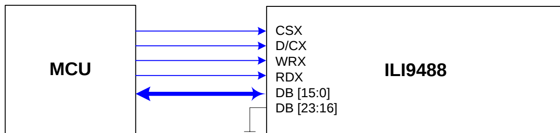
Figure 114: 16-bit Parallel MCU Interface
