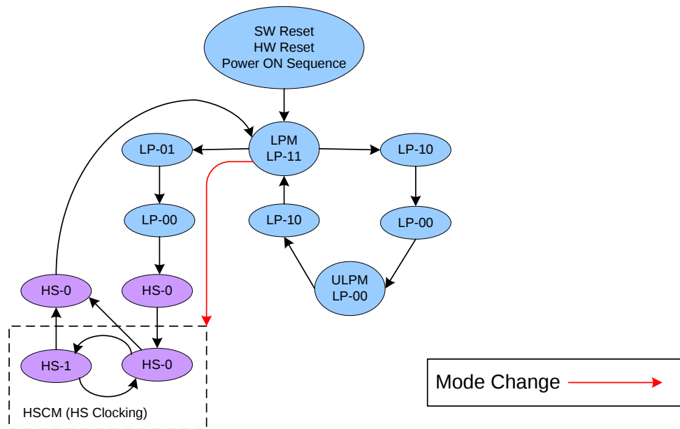
Figure 28: Mode Change from LPM to HSCM
