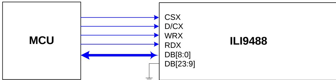
Figure 112: 9-bit Parallel MCU Interface
