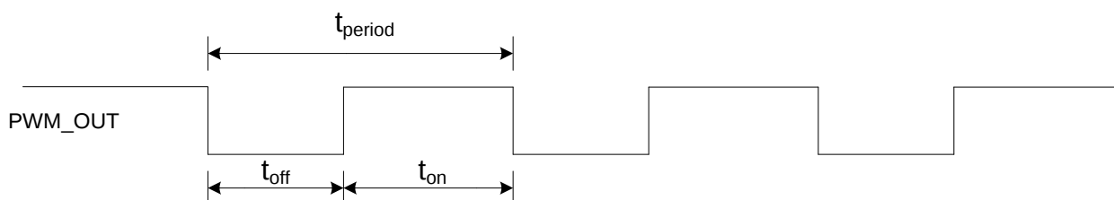
Figure 133: CABC_PWM On/Off Period
