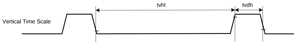
Figure 130: Tearing Effect Line Mode 1
