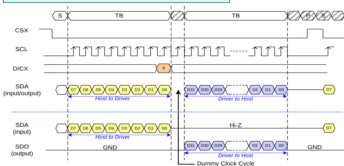
Figure 10: DBI Type C (Option 3) Read Cycle Sequence
