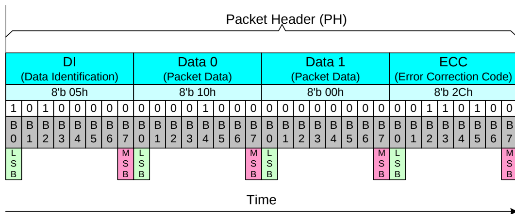
Figure 66: Display Command Set (DCS) Write, no Parameter (DCSWN-S) – Example
