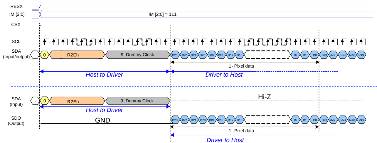
Figure 104: 3-Line SPI Mode Read Data
