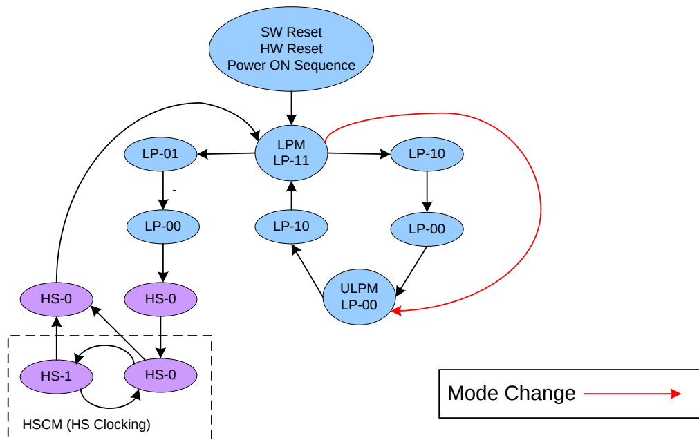
Figure 26: Mode Change from LPM to ULPM
