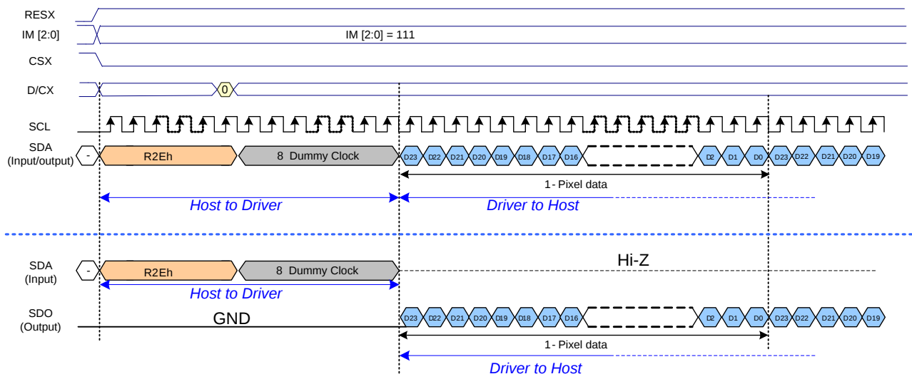
Figure 108: 4-Line SPI Mode Read Data
