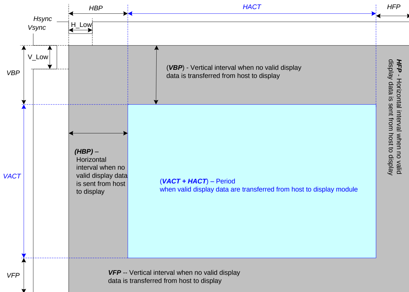
Figure 18: General DPI Timing Diagram
