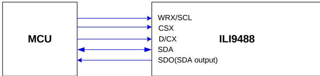
Figure 105: 4-Line Serial Interface
