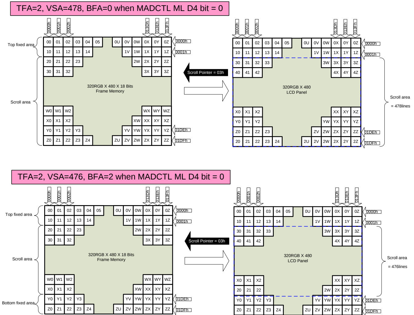
Figure 128: Vertical Scrolling Mode Function
