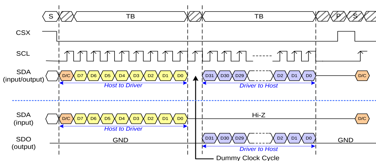
Figure 9: DBI Type C (Option 1) Read Cycle Sequence
