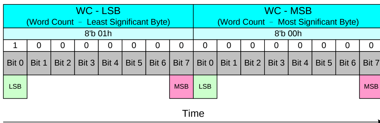
Figure 45: Byte Order of Multiple Byte Information in Packets
