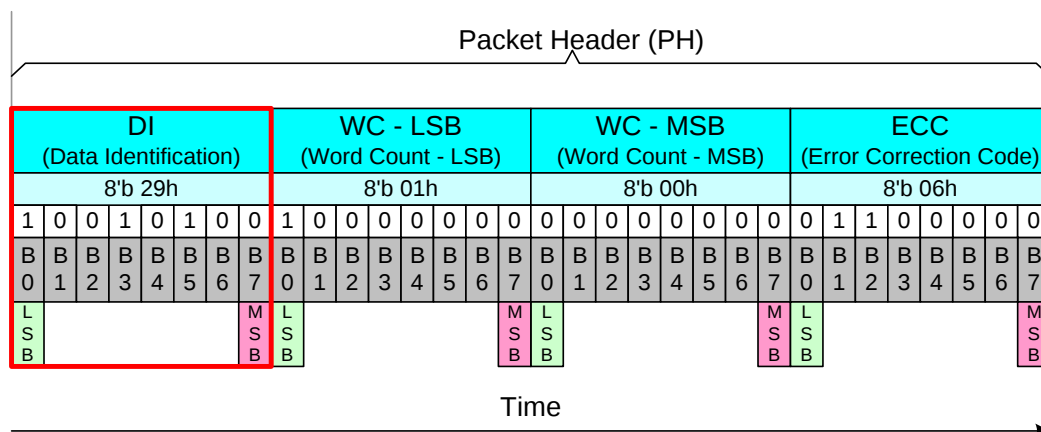
Figure 49: Data Identification (DI) of the Packet Header (PH)
