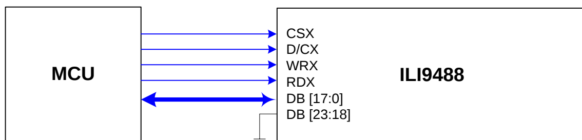
Figure 117: 18-bit Parallel MCU Interface
