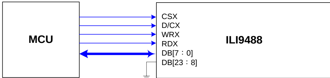
Figure 109: 8-bit Parallel MCU Interface
