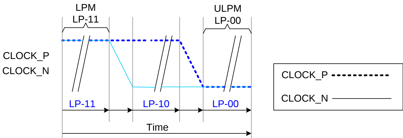
Figure 25: From LPM to ULPM
