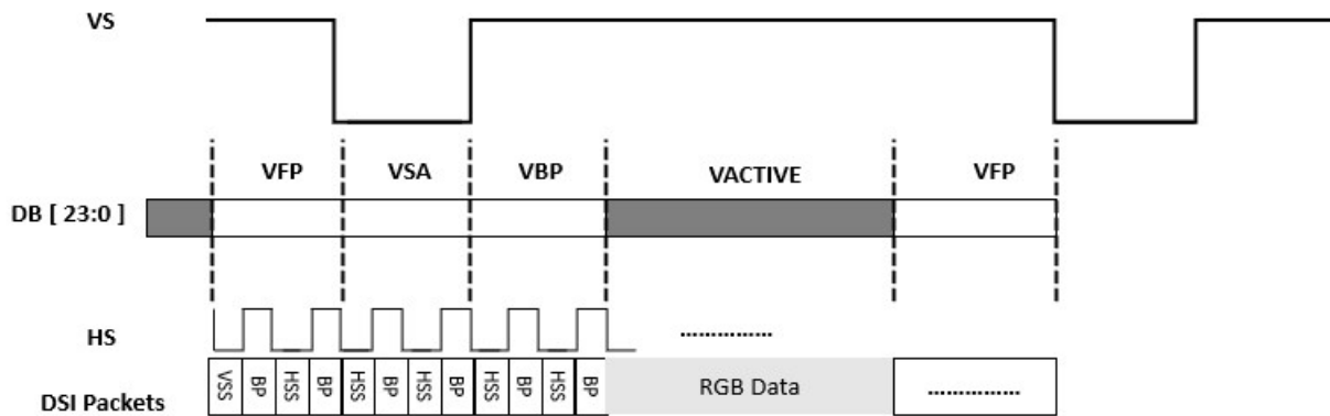
Figure 7.9: Vertical timings for DSI
