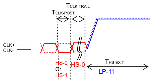
Figure 5-8: From High Speed Clock mode to LPM
