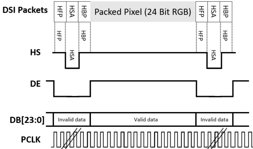
Figure 7.10: Horizontal timings for DSI
