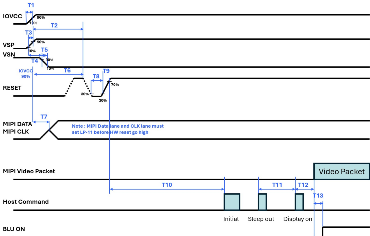
Figure 8-8: DSI Power On Sequence of 3 Power Mode
